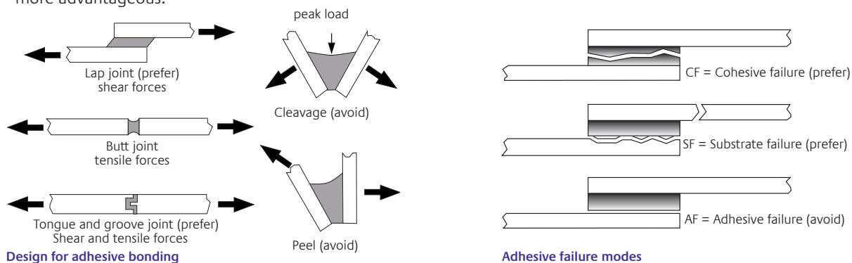
Design for adhesive bonding
